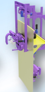
Floating Roof- External & Internal Support
